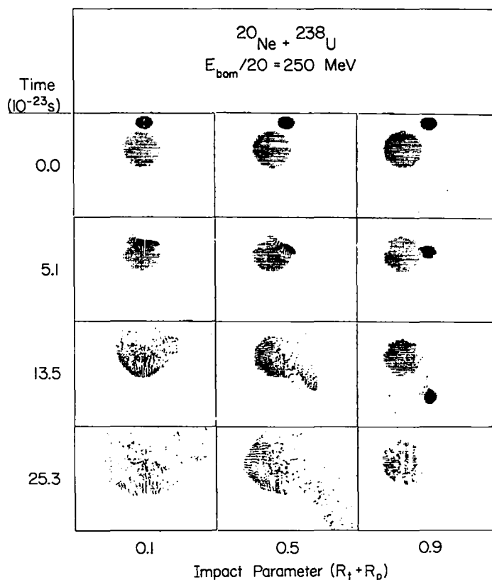
Time evolution of the matter distribution in the collision of ^{20}\text{Ne} with ^{238}\text{U} for three different impact parameters as calculated in a one-fluid hydrodynamical model by members of T-3 (Fluid Dynamics) and T-9 (Nuclear Theory). The laboratory bombarding energy per nucleon is 250 MeV. These and other studies of high-energy heavy ion collisions, where nuclear matter may be compressed to greater than normal densities, promise to yield information about the nuclear equation of state and the possible existence of "abnormal" or soliton-like states of nuclear matter. Members of T-5 and T-8 are also involved in these studies.
